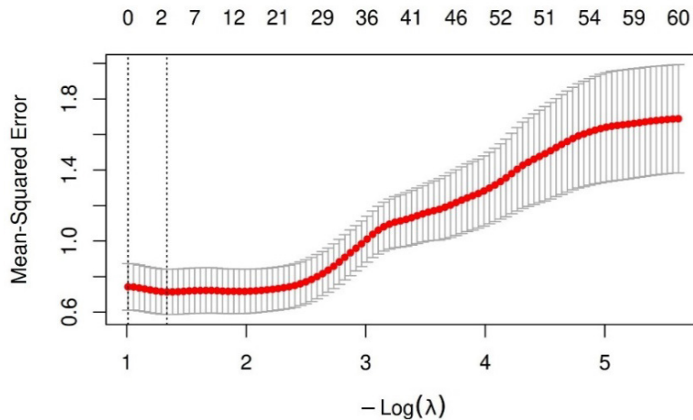
Figure A2 Selection of the optimal regularisation parameter \lambda in LASSO regression using 10-fold cross-validation.
