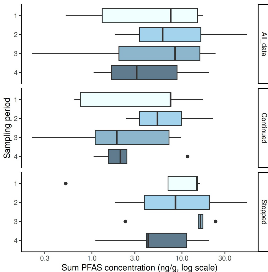
Figure 14 Sum of PFAS concentrations in home-produced eggs during the four sampling periods at ten locations.
