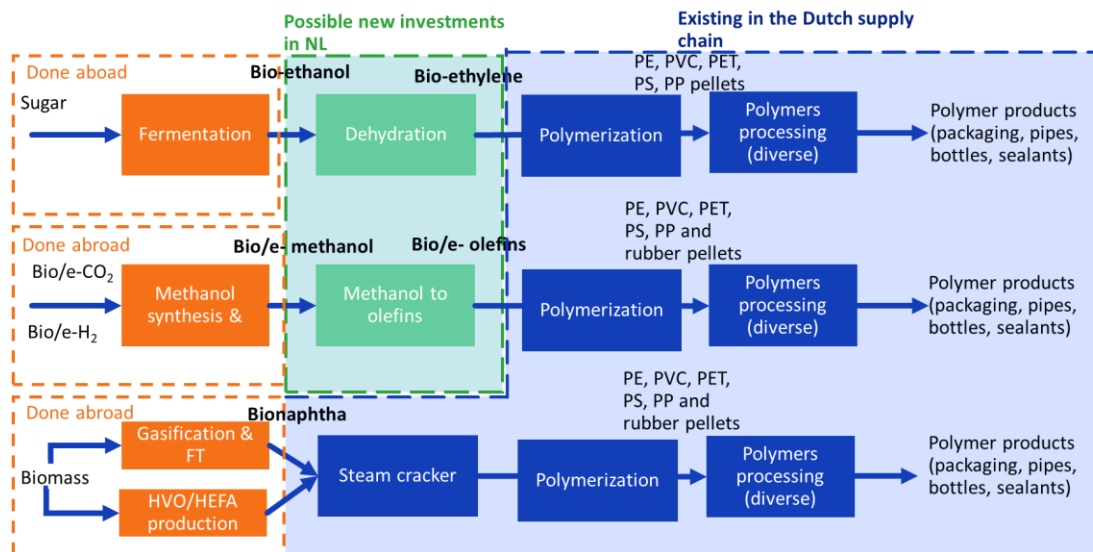
Figure 3.14: Renewable feedstock import alternatives
