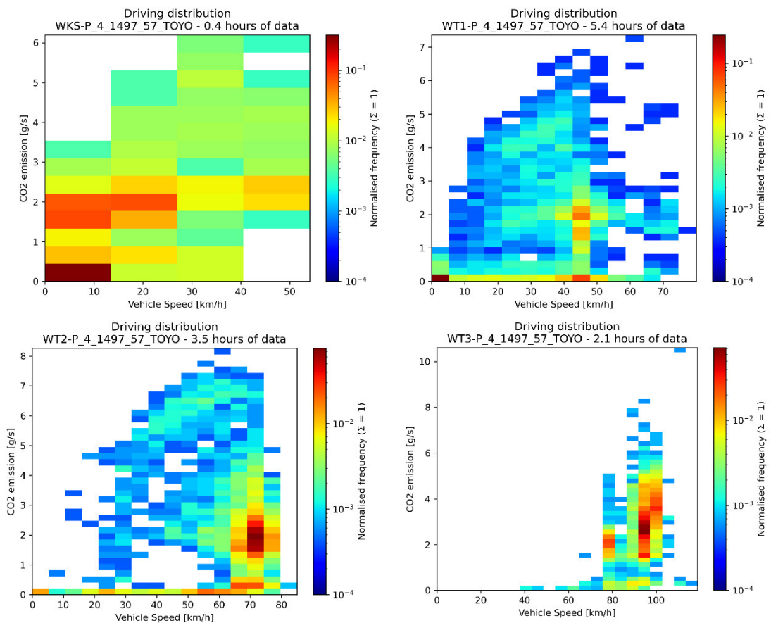
Figure A.4: Normalised frequency of \text{CO}_2 emissions and vehicle speed, where dark red indicates the area which occurs most often for the four road types now included in VERSIT+: WKS (cold start extra emissions in the first kilometre), WT1 (urban), WT2 (rural) and WT3 (motorway).
