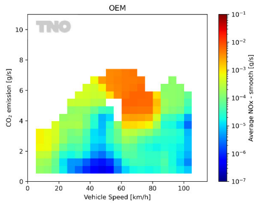
Figure A.3: Emission map of the \text{NO}_x emissions as a function of \text{CO}_2 and speed, of the Toyota Prius with the original OEM catalyst, as reproduced from Figure 3.2. Red indicates higher \text{NO}_x emissions; the localisation of these higher emissions demonstrates differences in catalytic function
