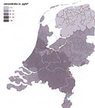
PM 10 , 2017
