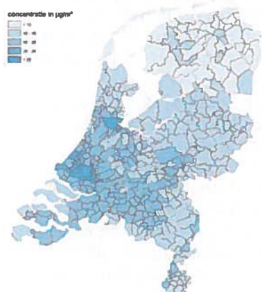
NO 2 , 2020 (prognose)
