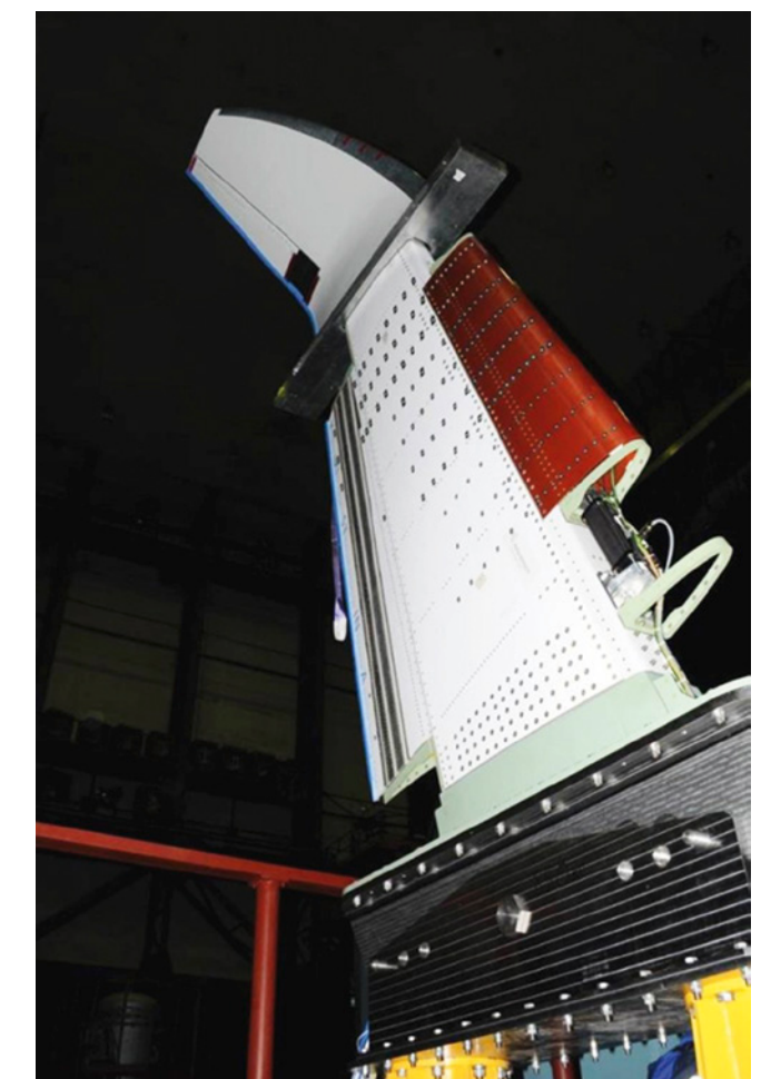
TANGO - AMF test in Hamburg
