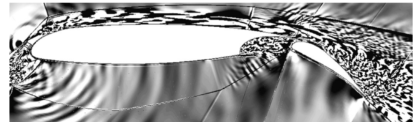
Advanced simulation of the flow dynamics around a three-element airfoil thanks to the ZDES technique developed by ONERA (adapted from Deck & Larauie, Journal of Fluid Mechanics, vol 723, pp 401-444, 2013)
